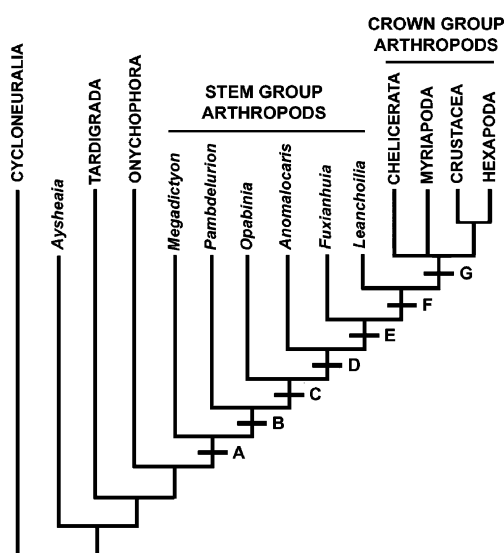
Fig. 3 Relationships of panarthropods including extinct taxa (names in italics , lower in the tree) and living taxa (names in upper case at the top of the tree). The series of fossils from Megadictyon to Leanchollia represent stem group Arthropoda, whereas all species descended from the most recent common ancestor of living chelicerates and insects or crustaceans are crown group arthropods. The letters A–G represent evolutionary events in the arthropod stem group, including: A paired, segmentally arranged midgut glands; B trunk appendage flaps in the form of lateral lobes; C trunk without annulation; D appendages having stiffened regions separated by soft membranes (=arthropodization); E hard, articulated tergal exoskeleton; F limb bases with spiny, gnathobasic endites; G locomotory limbs with only five to seven articles exclusive of terminal claw
