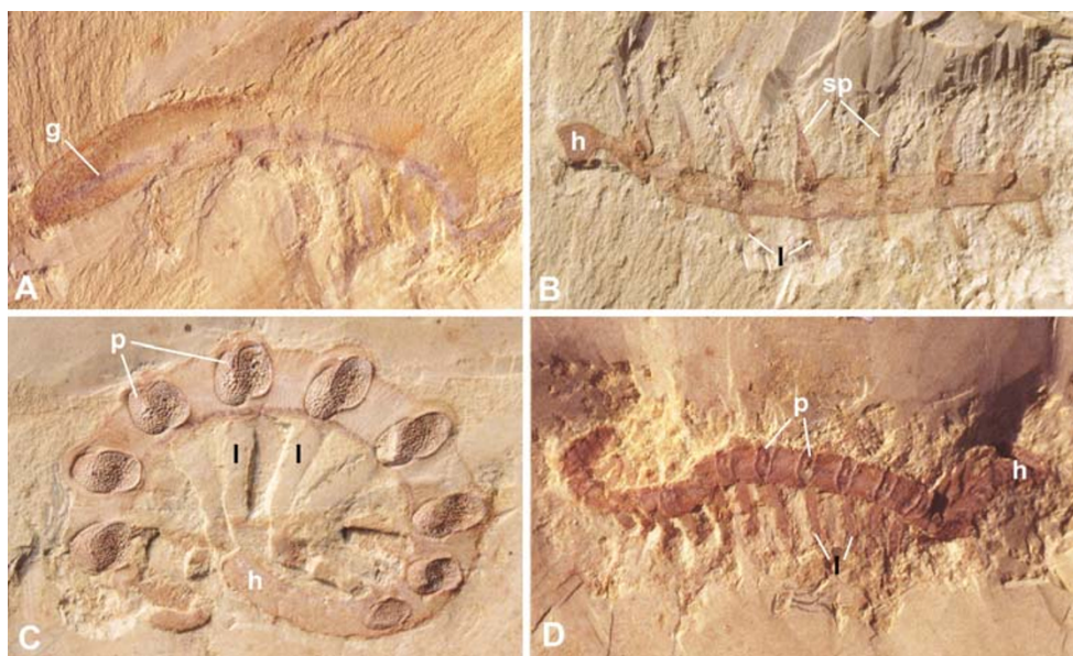
Fig. 4 Lobopodians from the early Cambrian Chengjiang Lagerstätte, China (photos by Lars Ramsköld). a Paucipodia inermis . b Hallucigenia fortis . c Microdictyon sinicum . d Cardiodictyon catenulum . g gut, h head, l legs/lobopods, p plates, sp spines
