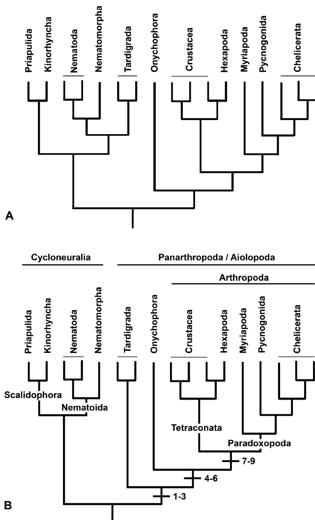
Fig. 2 Alternative hypotheses for ecdysozoan relationships based on molecular data from expressed sequence tags (after Dunn et al. 2008), depicting Panarthropoda as variably having multiple evolutionary origins ( a tardigrades within Cycloneuralia) or a single evolutionary origin ( b tardigrades sister to Onychophora + Arthropoda). Characters involving segmentation are mapped onto cladogram b as follows: 1 paired segmental ventrolateral appendages, 2 paired leg nerves, 3 Engrailed gene expressed in posterior ectoderm of each segment (Gabriel and Goldstein 2007), 4 segmented leg musculature (Schmidt-Rhaesa and Kulesa 2007), 5 commissures in ventral nerve cord (Zantke et al. 2008), 6 segmented nephridia (Mayer 2006), 7 commissures in ventral nerve cord in segmental register/rope-ladder nervous system (Mayer and Harzsch 2007), 8 segmented neurons show a reaction to serotonin (Mayer and Harzsch 2008), 9 Pax protein has a pair-rule function (Gabriel and Goldstein 2007)
