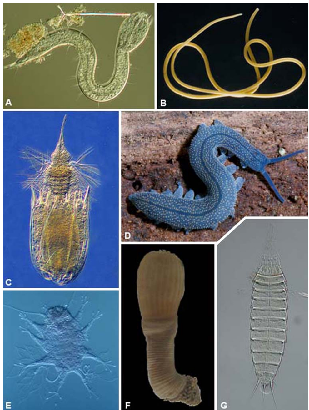
Fig. 1 Examples of the phyla of molting animals grouped with arthropods in Ecdysozoa.
